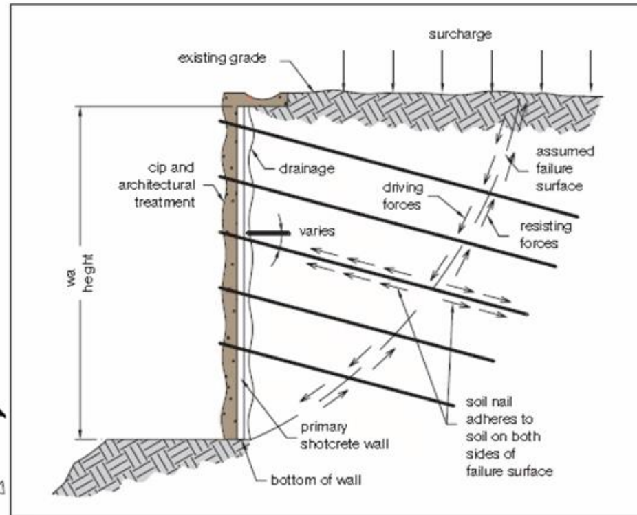
Typical section — Soil Nail Retaining Wall
